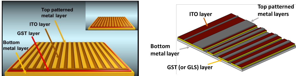
Fig. 1: (a) (left) Typical structure of a phase-change meta-absorber/modulator type device (inset shows a polarisation insensitive design). (b) (right) Typical structure of a phase-change meta beam steering device.
