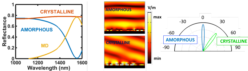
Fig. 2: (a) (left) Reflectance spectrum for a GST-based modulator device of the form shown in Fig. 1(a). (b) (right) Scattered electric field profile and far-field radiation pattern for a GLS-based beam steering device similar to that shown in Fig. 1(b).
